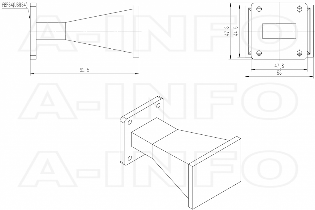
FBP84 Output with Radome (Option, P/N: LB-112-10-ASPO, Outdoor Application)
